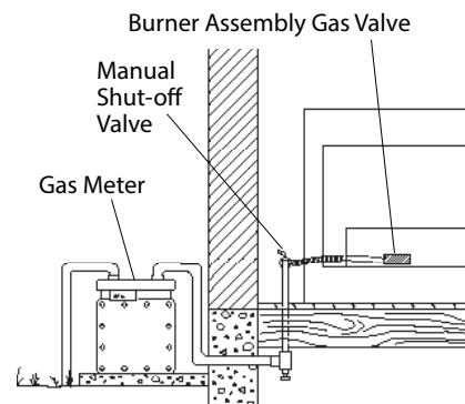
Equipment Shut-off Valve
