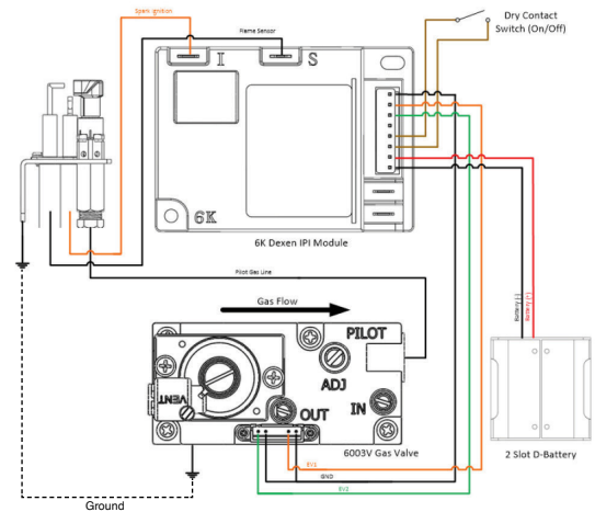
6003V - Battery Powered IPI System (6K)
