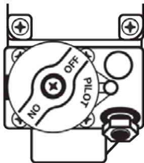
“PILOT” POSITION
